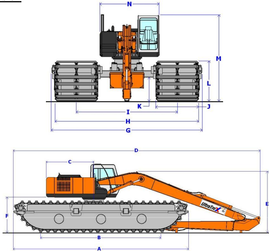
AT300 Amphibious Hydraulic Excavator
